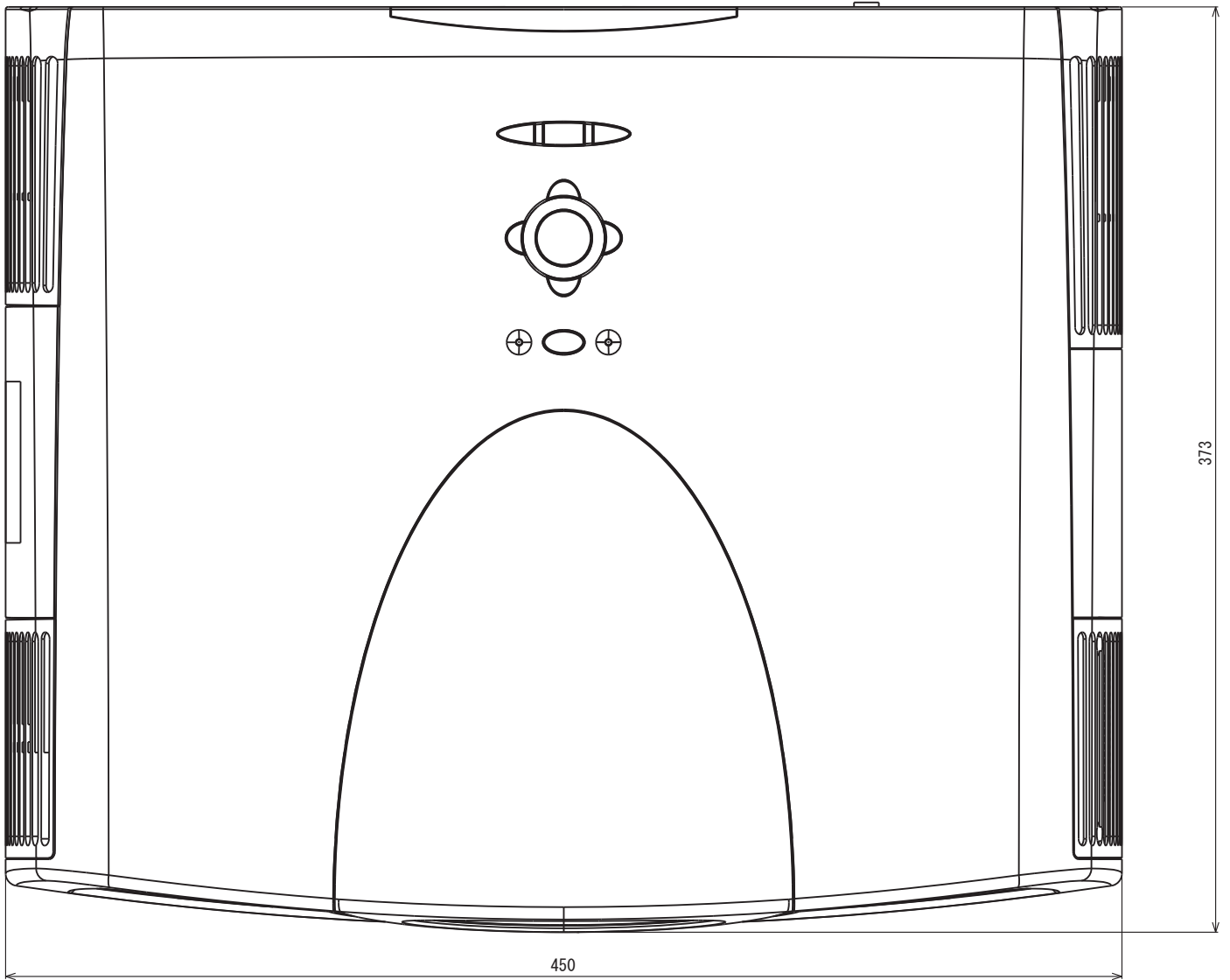
TOP VIEW (Detached Cover-Terminal)
